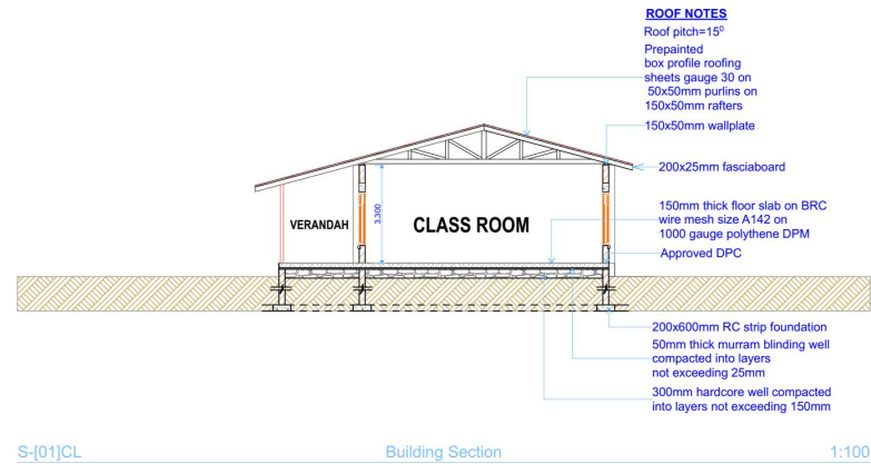
S-01|CL Building Section 1:100
