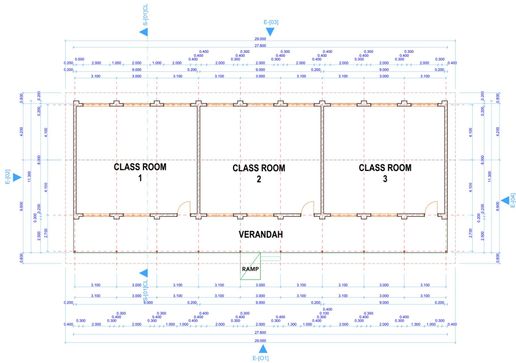
0. Ground Floor 1:100
